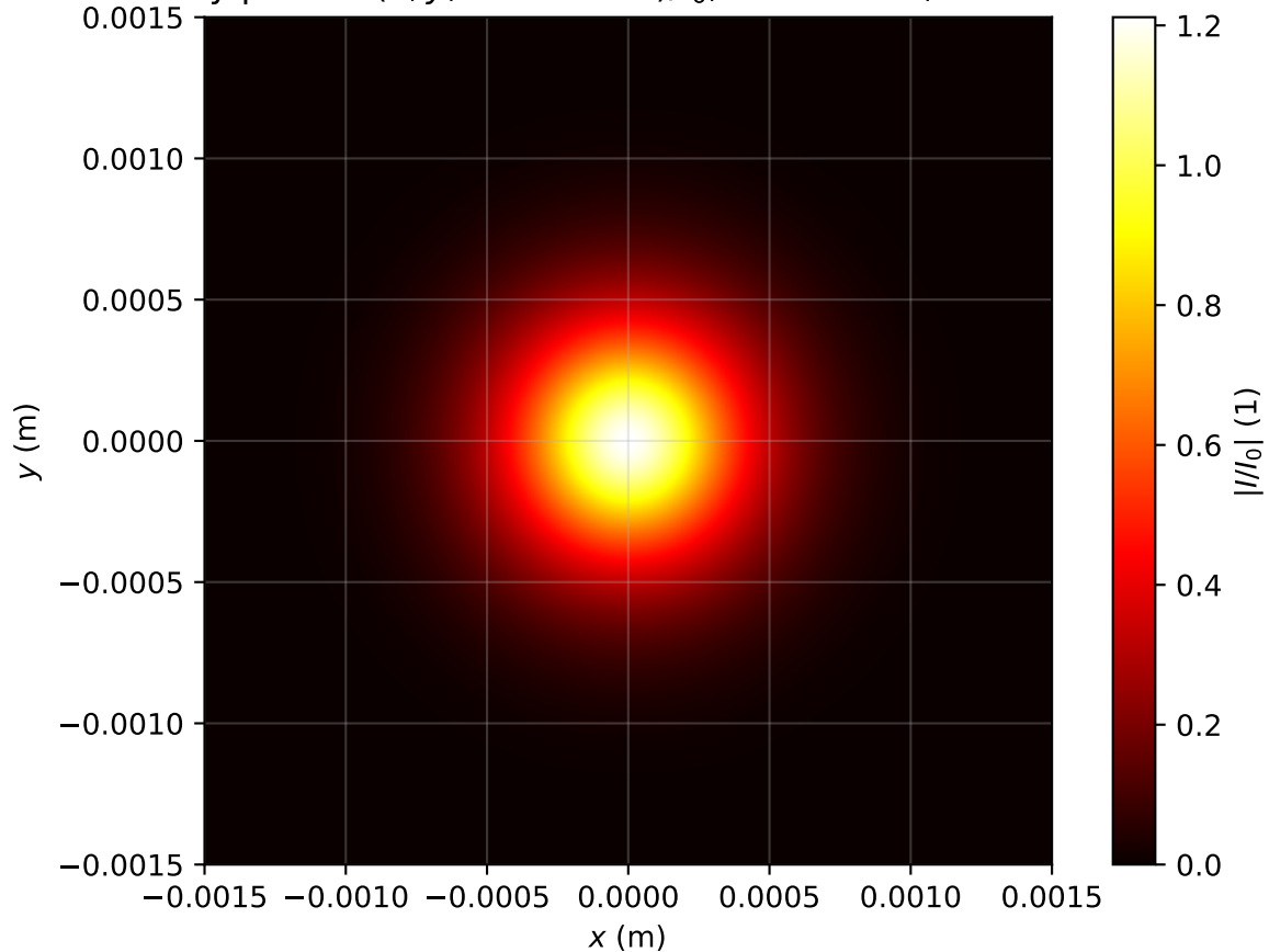
Intensity profile I(x, y, z = 0.557m)/I_0 , Pin=1.0Pcr, artificial time
